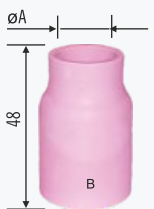
LARGE DIA LENS NOZZLE 57 N XX & 53 N XX
