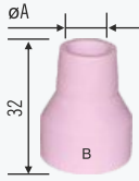
ARGON ARC NOZZLE 14 N XX
